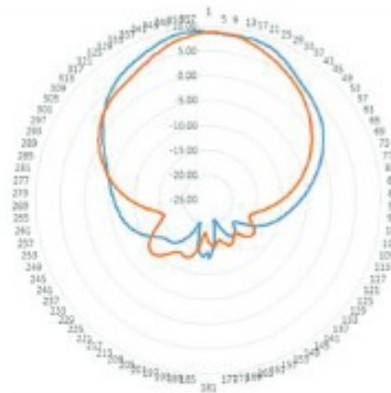
5 GHz Antenna Radiation Pattern
